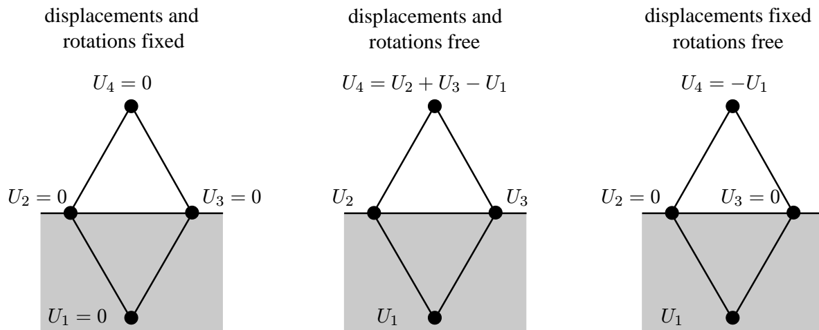
Figure 12: Boundary conditions.
