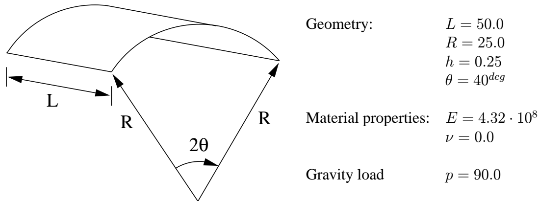
Figure 16: Definition of Scordelis-Lo problem.
