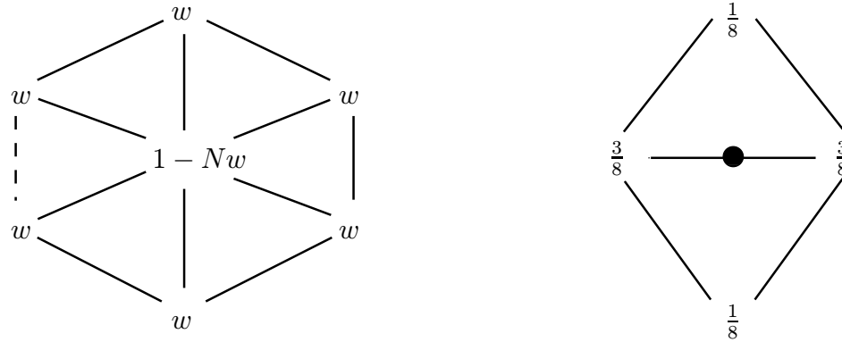
Figure 5: Refinement mask for Loop's subdivision scheme.
