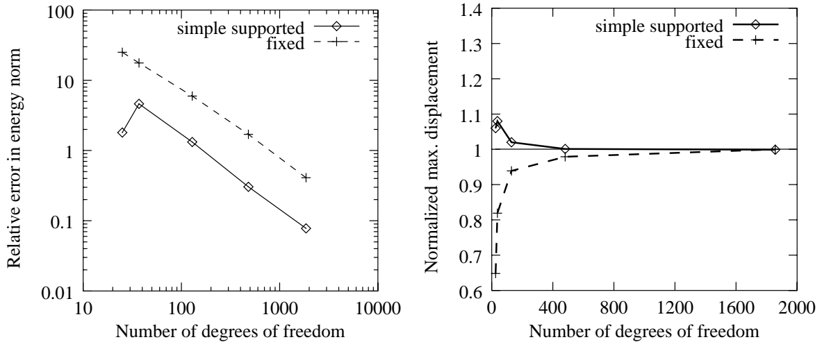
Figure 15: Convergence of the energy and maximum-displacement errors for the simply-supported and clamped plate problems.
