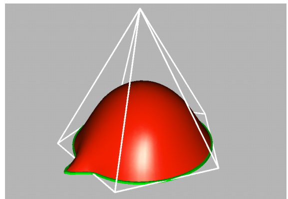
Figure 16: Introducing small perturbations to the given curves results in small and local perturbations of the limit surface. Notice that the original control net does not contain the information of the small perturbations. These come directly from the data of the curves.
