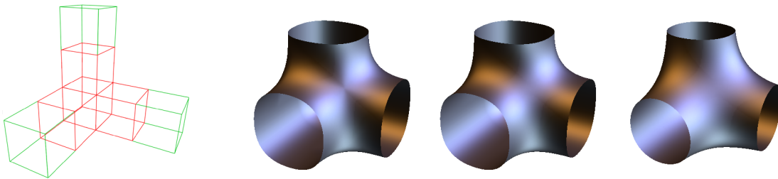
Figure 4.24: Control mesh for a three legged pipe (left). The red parts denote the control mesh for Midedge and Doo-Sabin, while the additional green section is necessary to have a complete set of boundary conditions for the bi-quartic scheme. The resulting surfaces in order: Midedge, Doo-Sabin, and Biquartic. Note the pinch point visible for Midedge and the increasing smoothness and roundness for Doo-Sabin and Biquartic.
