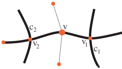
Figure 7: A regular boundary c-vertex between two boundary intersection vertices
