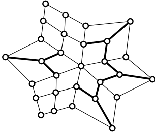
Figure 19: Combination of Y-elements
