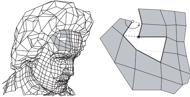
FIG. 5 The black vertex demonstrates the split situation. This vertex already exists in a visited region, but the current (dashed) face cannot find it from its immediate neighbors.
