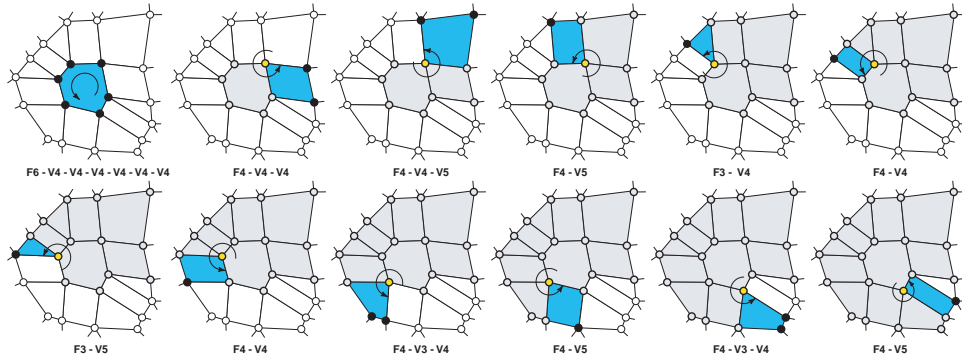
FIG. 3 Example of a simple traversal sequence starting from a seed face. At the beginning, the seed face degree is output along with the valence of all its vertices. The first vertex then becomes active and the next face is traversed in counterclockwise order, resulting in one face degree and two vertex valences output. The traversal keeps going until all the faces and vertices have been visited.
