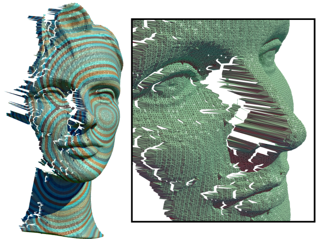
Fig. 17. Smoothed geodesic distance on an extremely poor triangulation with significant noise – note that small holes are essentially ignored. Also note good approximation of distance even along thin slivers in the nose.
