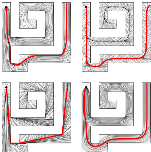
Fig. 12. For path planning, the behavior of geodesics can be controlled via boundary conditions and the time step t . Top-left : Neumann conditions encourage boundary adhesion. Top-right : Dirichlet conditions encourage avoidance. Bottom-left : small values of t yield standard straight-line geodesics. Bottom-right : large values of t yield more natural trajectories.
