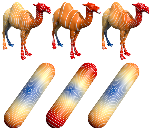
Fig. 10. Top row : our smoothed approximation of geodesic distance (left) and biharmonic distance (center) both mitigate sharp “cusps” found in the exact distance (right), yet isoline spacing of the biharmonic distance can vary dramatically. Bottom row : biharmonic distance (center) tends to exhibit elliptical level lines near the source, while our smoothed distance (left) maintains isotropic circular profiles as seen in the exact distance (right). Camel mesh courtesy AIM@Shape.
