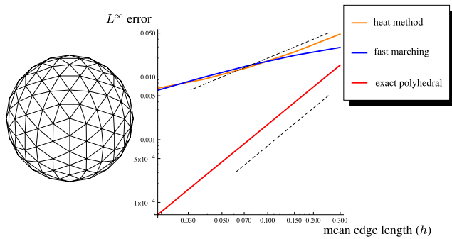
Fig. 21. L^\infty convergence of distance functions on the unit sphere with respect to mean edge length. As a baseline for comparison, we use the exact distance function \phi(x, y) = \cos^{-1}(x \cdot y) . Linear and quadratic convergence are plotted as dashed lines for reference; note that even the exact polyhedral distance converges only quadratically.
