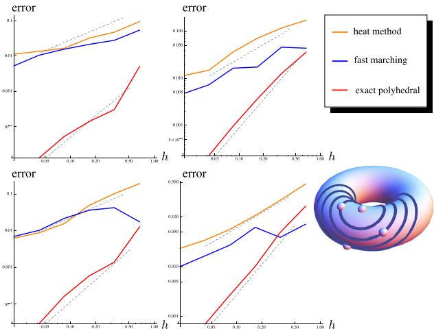
Fig. 22. Convergence of geodesic distance on the torus at four different test points. Error is the absolute value of the difference between the numerical value and the exact (smooth) distance; linear and quadratic convergence are plotted as dashed lines for reference. Right : test points visualized on the torus; dark blue lines are geodesic circles computed via Clairaut’s relation.
