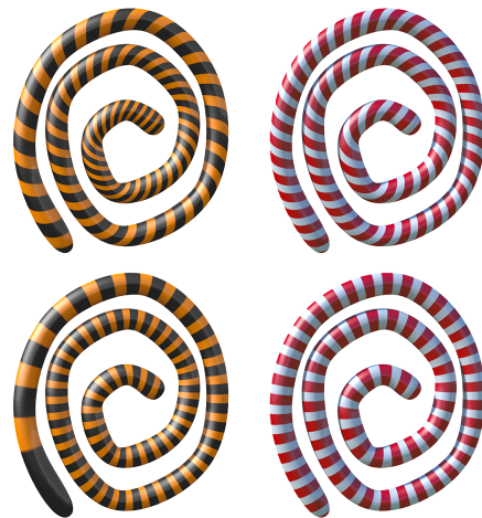
Fig. 6. Left : Varadhan’s formula. Right : the heat method. Even for very small values of t , simply applying Varadhan’s formula does not provide an accurate approximation of geodesic distance (top left); for large values of t spacing becomes even more uneven (bottom left). Normalizing the gradient results in a more accurate solution, as indicated by evenly spaced isolines (top right), and is also valuable when constructing a smoothed distance function (bottom right).
