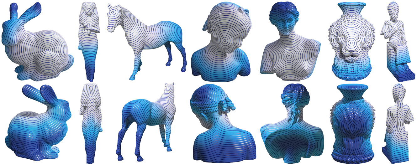
Fig. 13. Meshes used in Table I. Left to right: BUNNY, ISIS, HORSE, BIMBA, APHRODITE, LION, RAMSES 1 .
