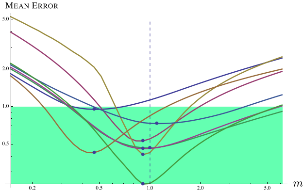
Fig. 20. Mean percent error as a function of m , where t = mh^2 . Each curve corresponds to a data set from Table I. Notice that in most examples m = 1 (dashed line) is close to the optimal parameter value (blue dots) and yields mean error below 1%.
