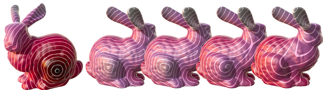
Fig. 9. A source on the front of the Stanford Bunny results in nonsmooth cusps on the opposite side. By running heat flow for progressively longer durations t , we obtain smoothed approximations of geodesic distance ( right ).
