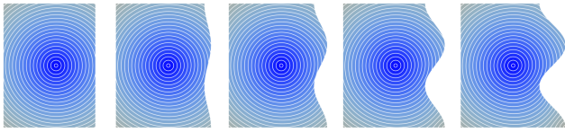
Fig. 19. Smoothed geodesic distance ( m = 1000 ) using “averaged” boundary conditions. Notice that increasing geodesic curvature along the boundary does not strongly influence the behavior of the solution.
