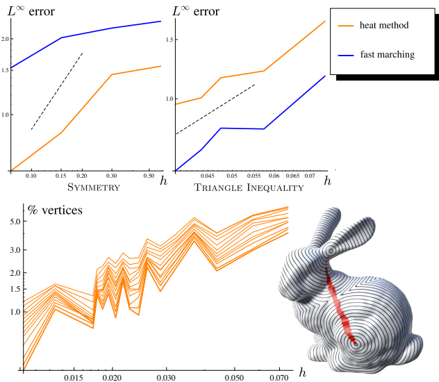
Fig. 23. Fast marching and the heat method both exhibit small violations of metric properties such as symmetry ( top left ) and the triangle inequality ( top right ) that vanish under refinement – we plot the worst violation among all pairs or triples of vertices (respectively) as a percent of mesh diameter. Dashed lines plot linear convergence. Bottom right : the triangle inequality is violated only for vertices along a geodesic between two distinguished points (in red), since the corresponding geodesic triangles are nearly degenerate. Bottom left : percent of red vertices as a function of h – each curve represents a different value of m sampled from the range [1, 100] .
